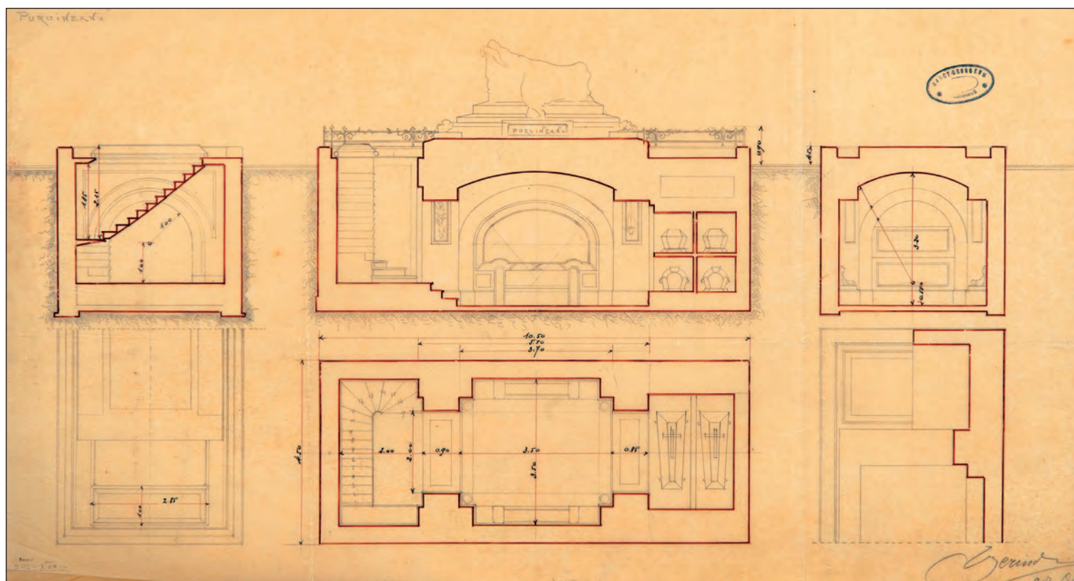
Fig. 1 - Cavoul familiei Poroineanu – proiect arh. I. Berindei 1908/Poroineanu family crypt – designed by arch. I. Berindei 1908. Arhiva MNAR - inv. 379/112.371
